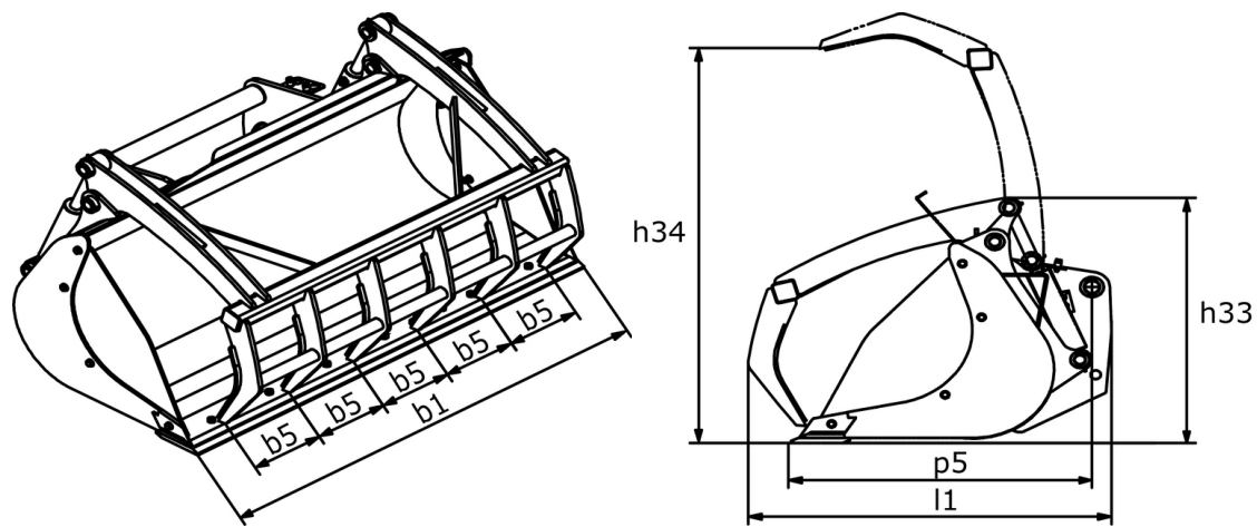
Agricultural Multifunction Grab Bucket - FO - Dimensional drawing
