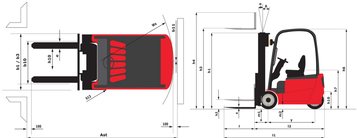
ME 315 C FOB - Diagrama dimensional
