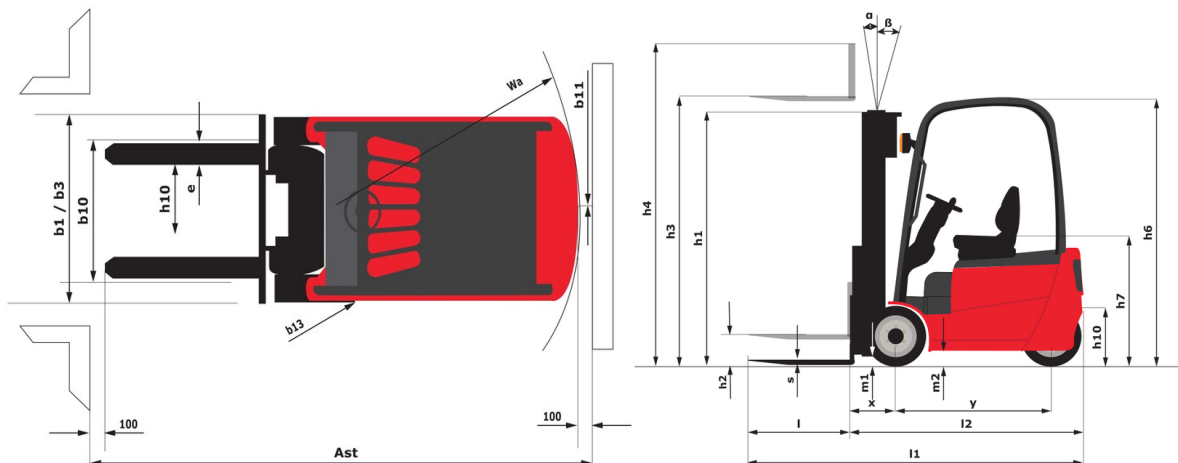
ME 315 FOB - Dimensional drawing
