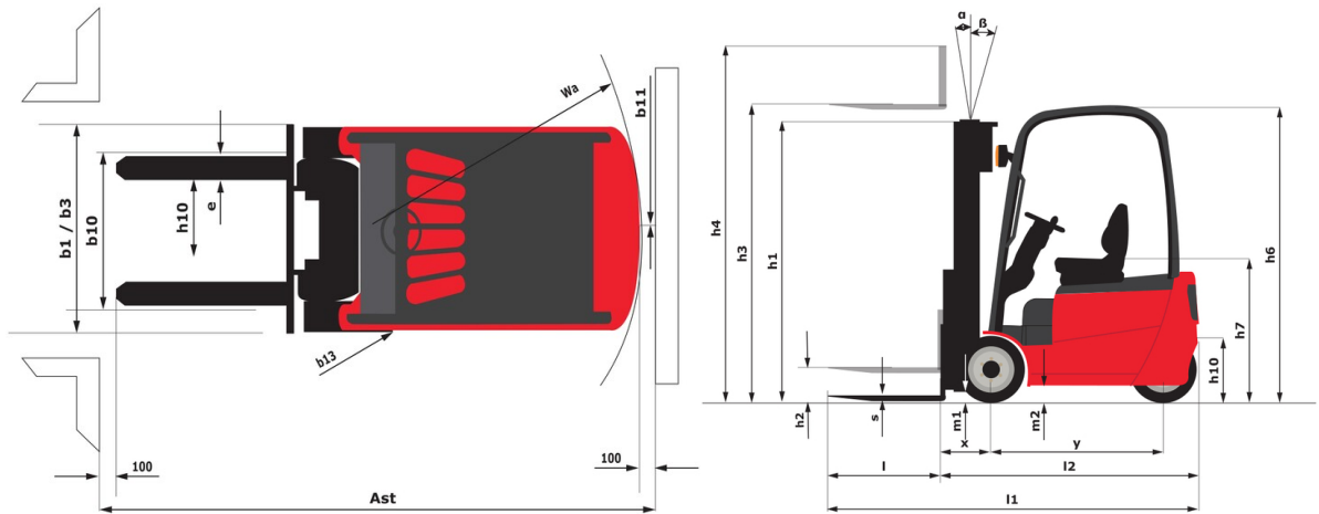
ME 420 FOB - Diagrama dimensional
