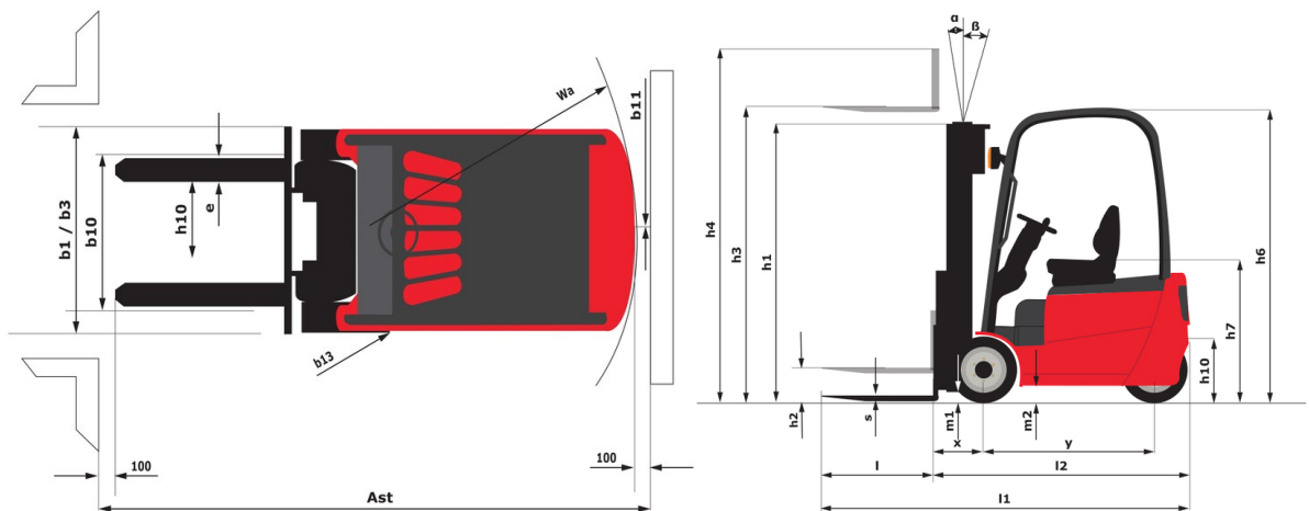
ME 425C FOB - Dimensional drawing
