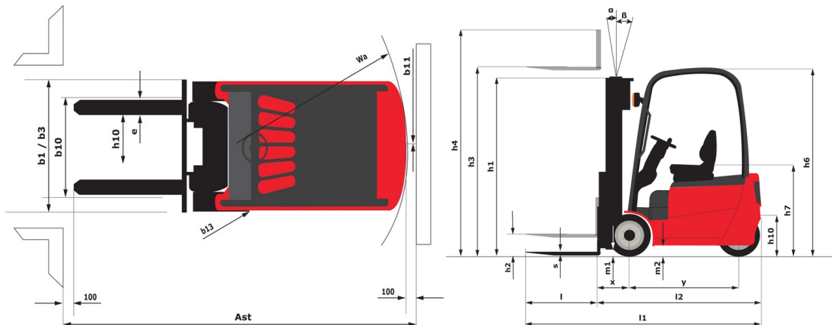
ME 440 FOB - Dimensional drawing
