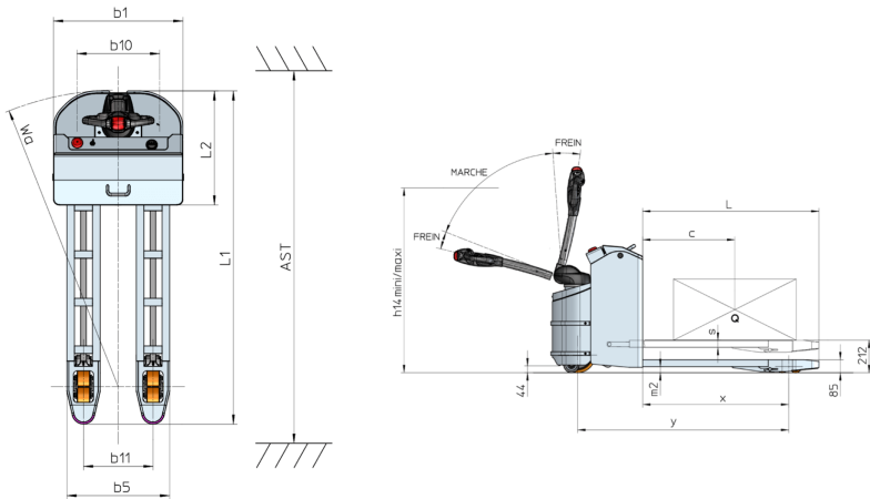
EP 20 Inox Premium - Dimensional drawing
