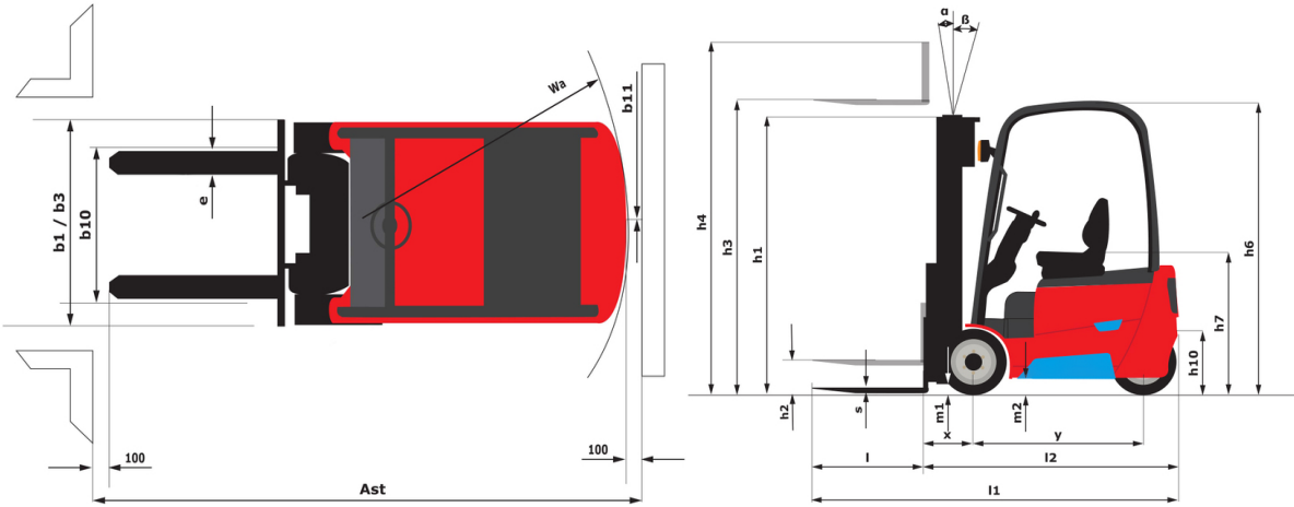
ME 316 LIFT - Dimensional drawing
