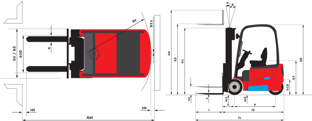
ME 316 LIFT - Dimensional drawing
