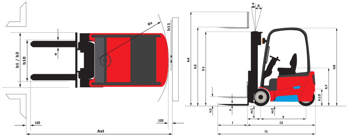
ME 320 LIFT - Diagrama dimensional
