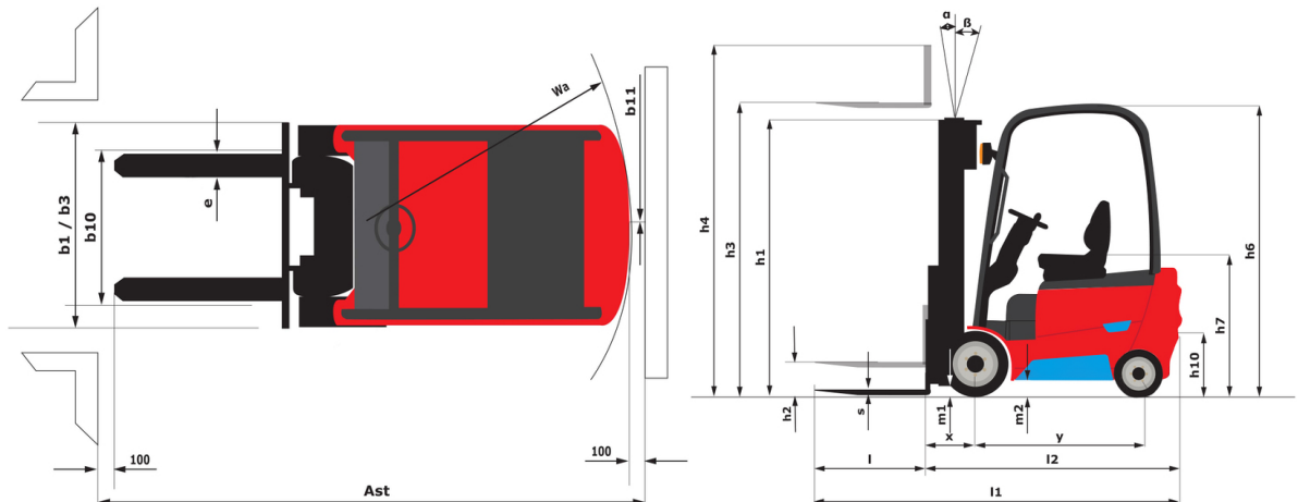
ME 425 LD LIFT - Dimensional drawing
