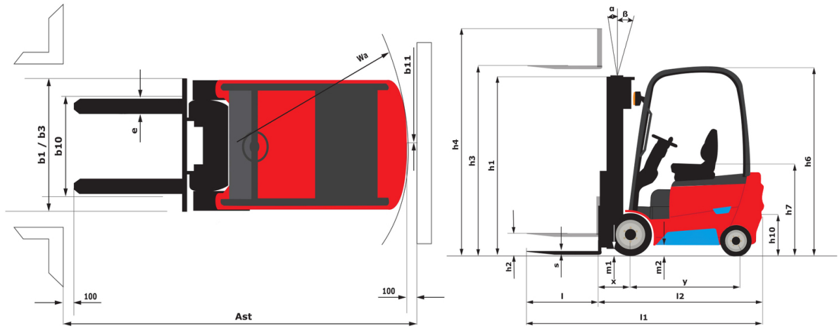
ME 430 LIFT - Diagrama dimensional
