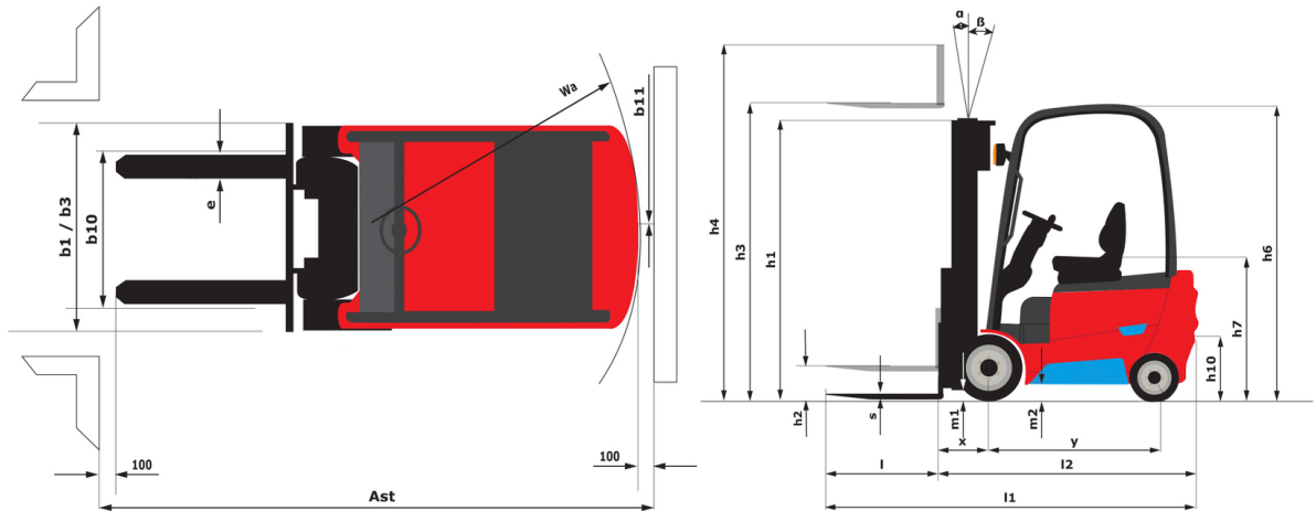
ME 430 LIFT - Diagrama dimensional
