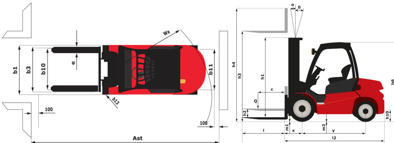
MI 80 D ST5 - Dimensional drawing
