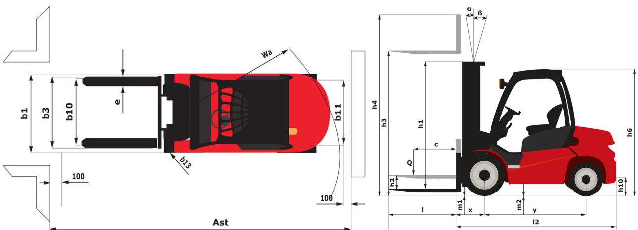
MI 50 LD ST5 FOB - Dimensional drawing
