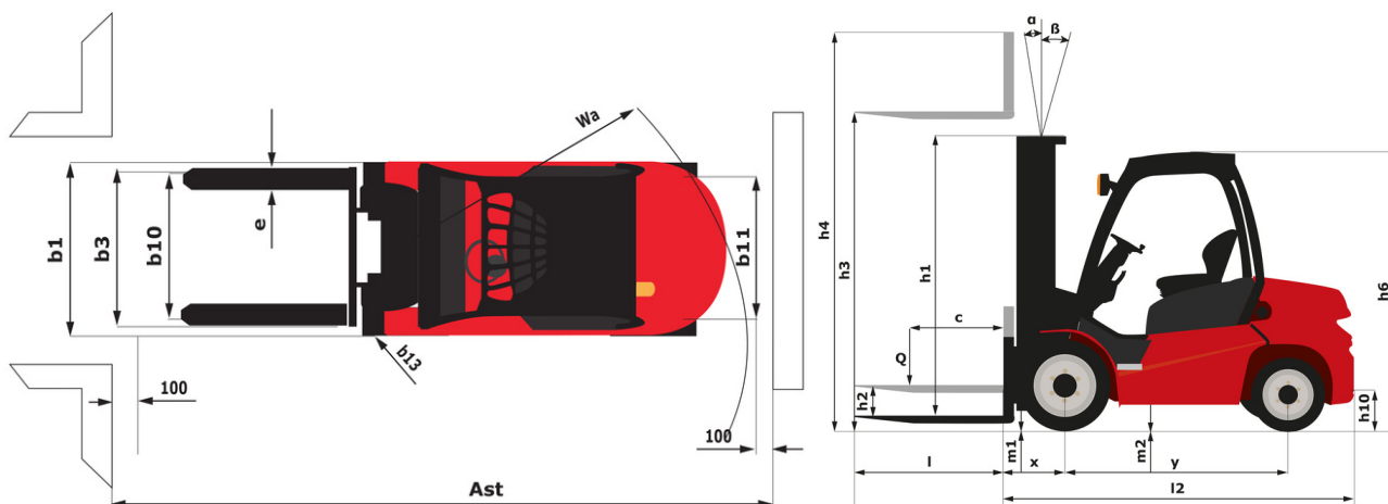
MI-X 40 D FOB - Dimensional drawing
