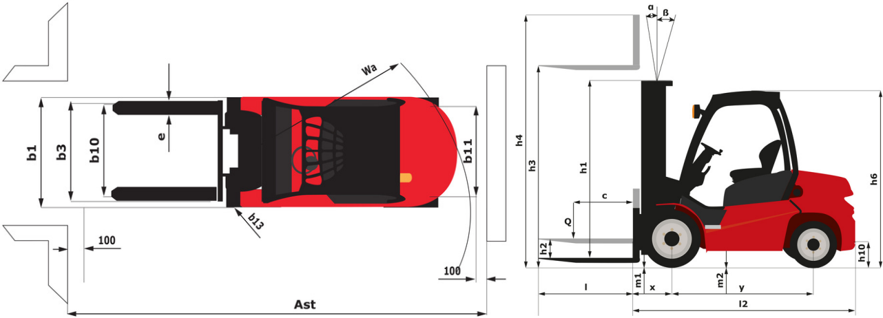
MI-X 55 D - Dimensional drawing
