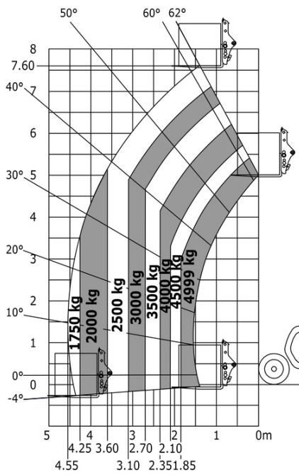
Machine on tires with forks Metric
