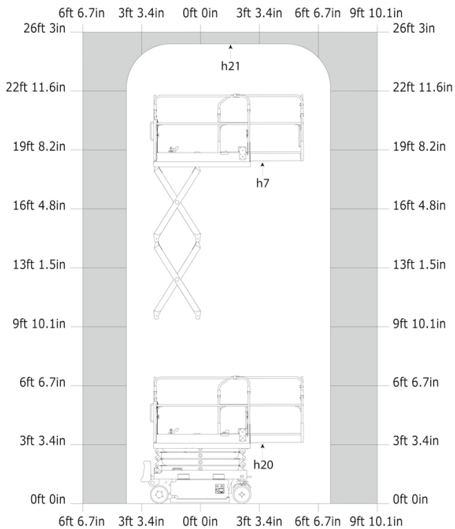
Load Chart for MEWP (Imperial)
