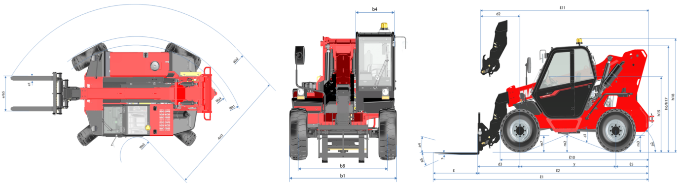
MXT 840 K IND (BSV) - Dimensional drawing
