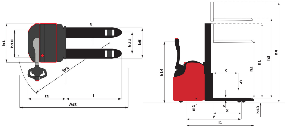
ES 725 - Dimensional drawing
