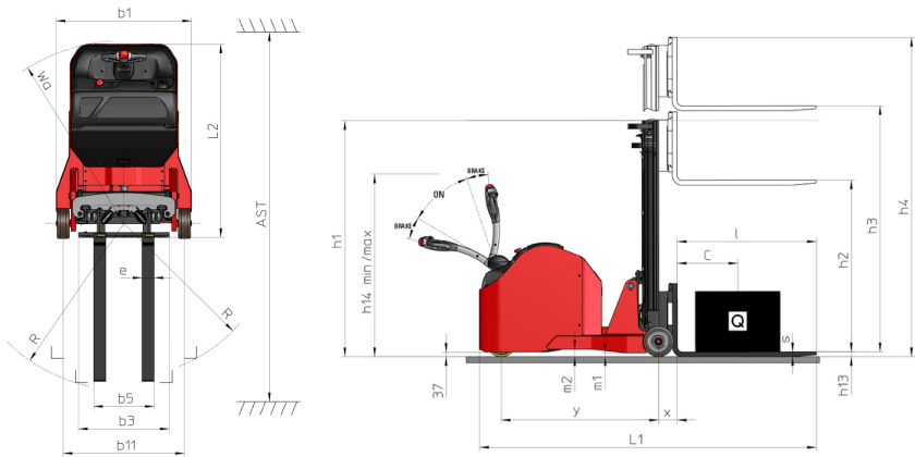
ES-C 716 - Dimensional drawing
