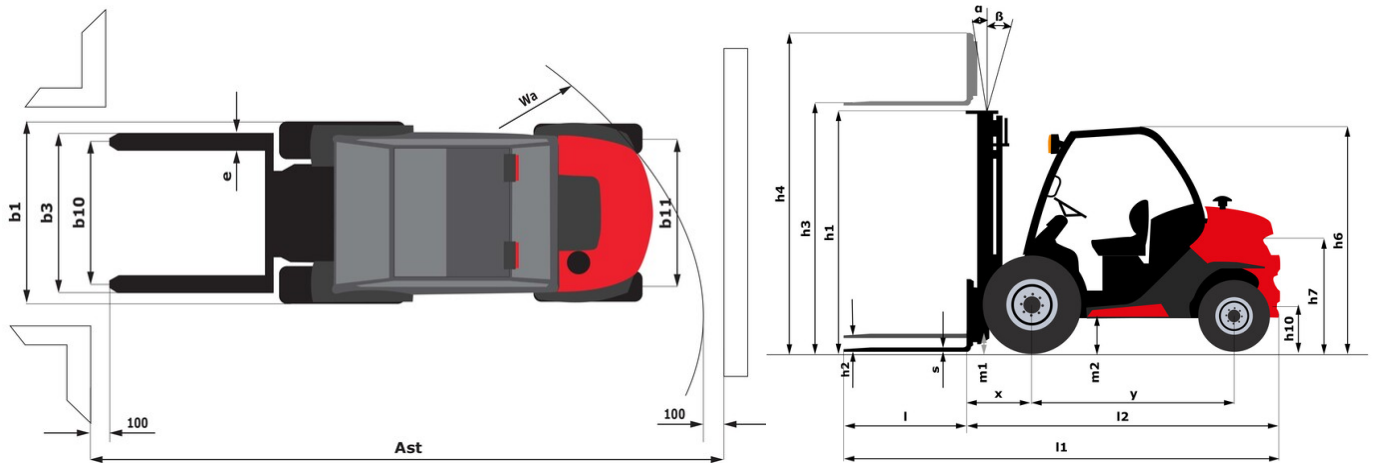
MC-X 18-4 - Dimensional drawing
