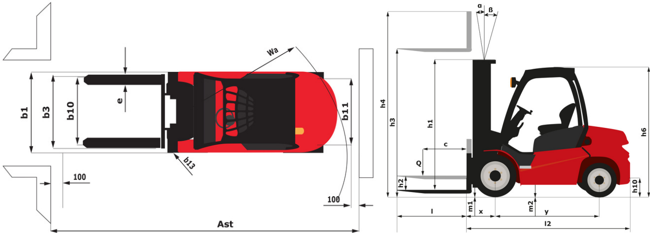
MI-X 15 D - Diagrama dimensional
