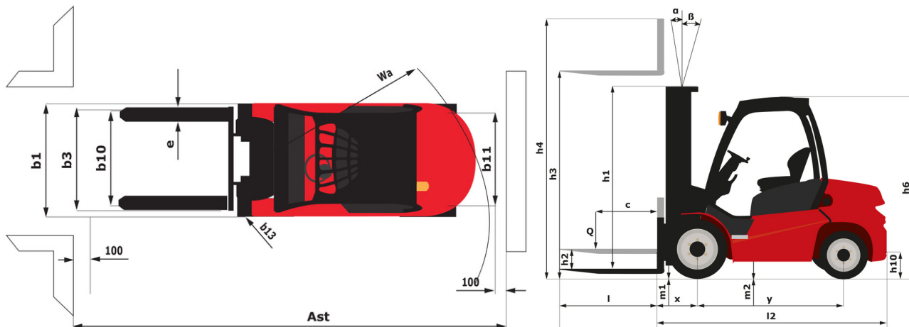
MI-X 15 G - Diagrama dimensional
