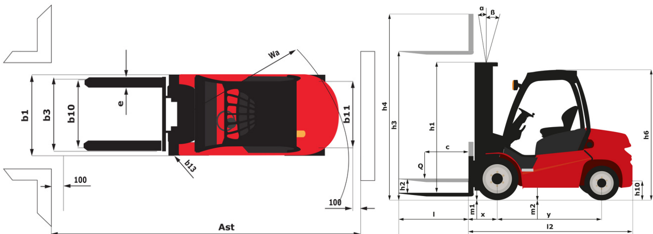
MI-X 20 G - Dimensional drawing
