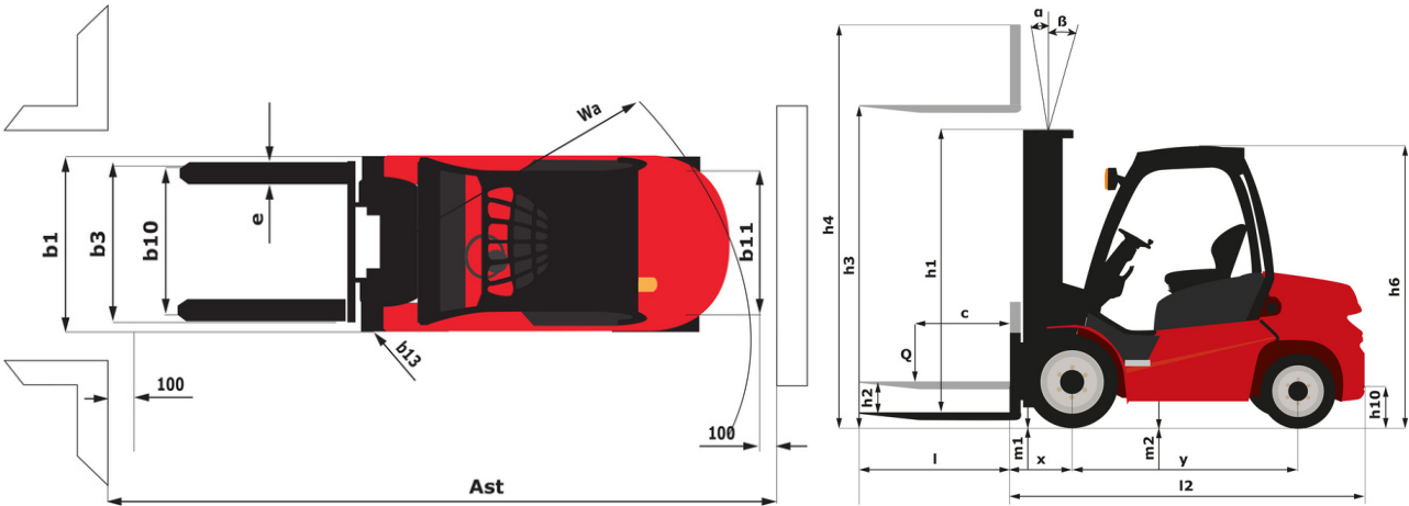
MI-X 20 G - Diagrama dimensional
