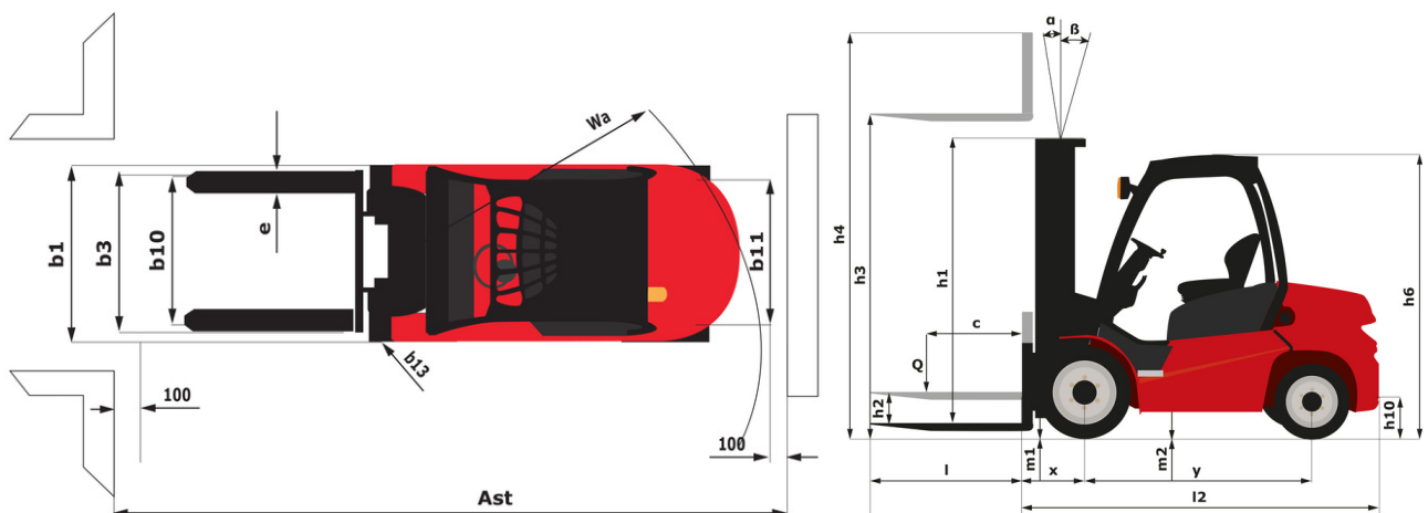
MI-X 25 G - Diagrama dimensional
