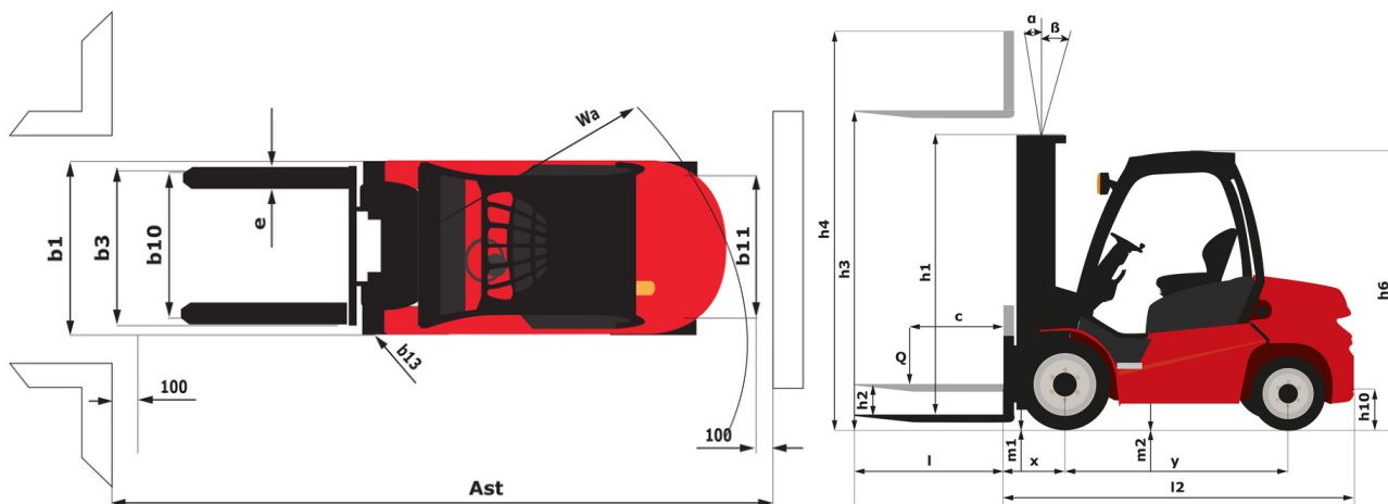
MI-X 30 D - Dimensional drawing
