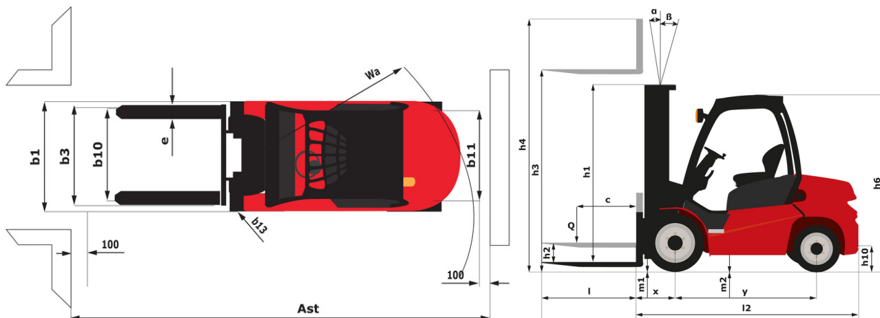
MI-X 30 G - Dimensional drawing
