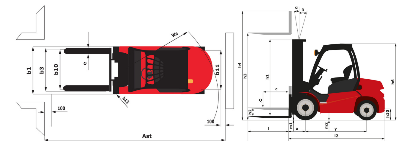
MI-X 35 G - Diagrama dimensional
