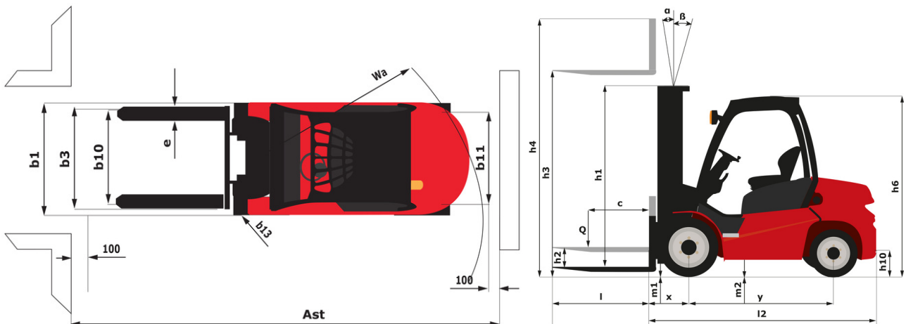
MI 25 D ST5 - Dimensional drawing
