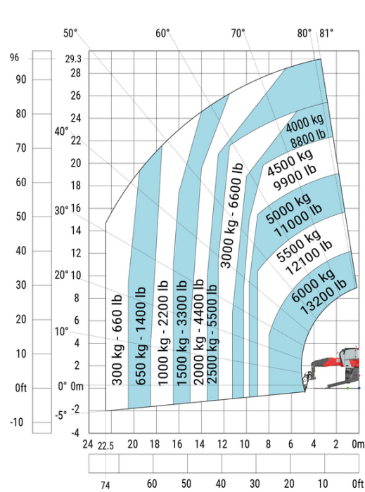
Machine on lowered stabilisers with winch 6000 kg (Imperial)
