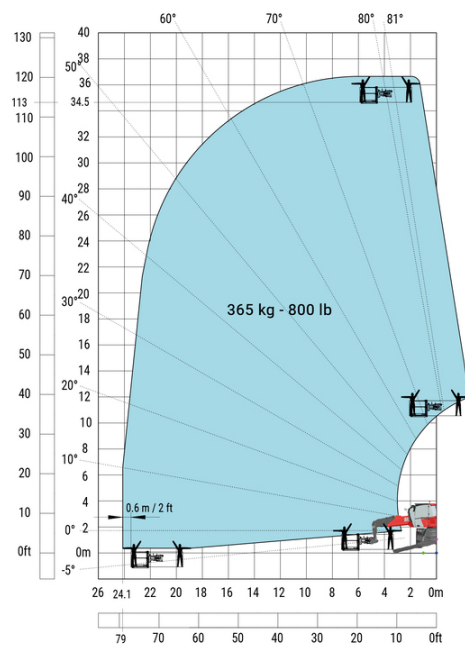
Machine on lowered stabilisers with hook 9000 kg (Metric) Machine on lowered stabilisers with 365 kg platform Metric
