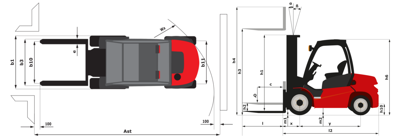
MSI-X 25 - Dimensional drawing
