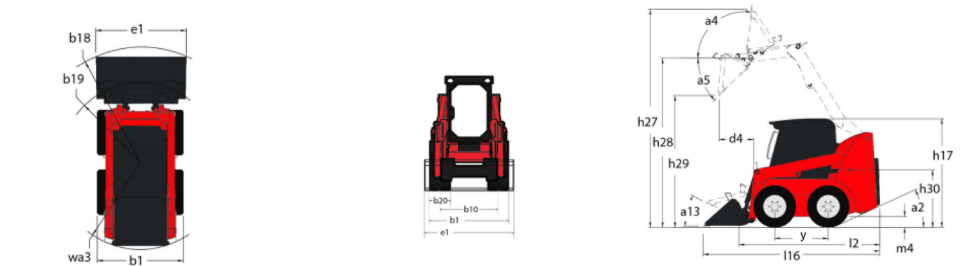
2100V - Diagrama dimensional
