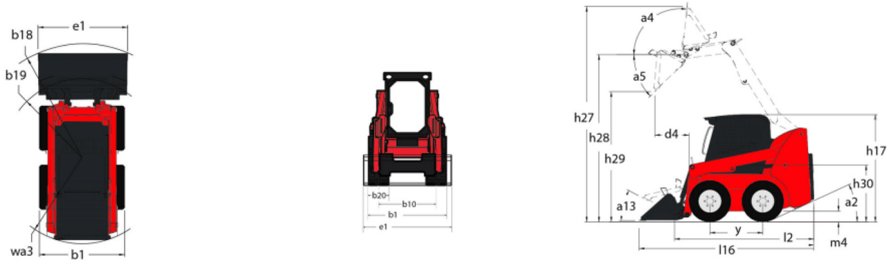
2300V - Dimensional drawing
