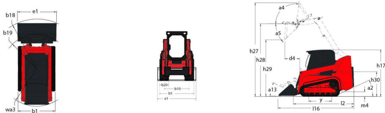
2300VT - Dimensional drawing
