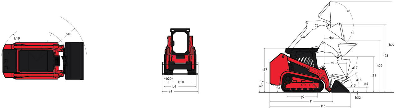
1650RT - Dimensional drawing
