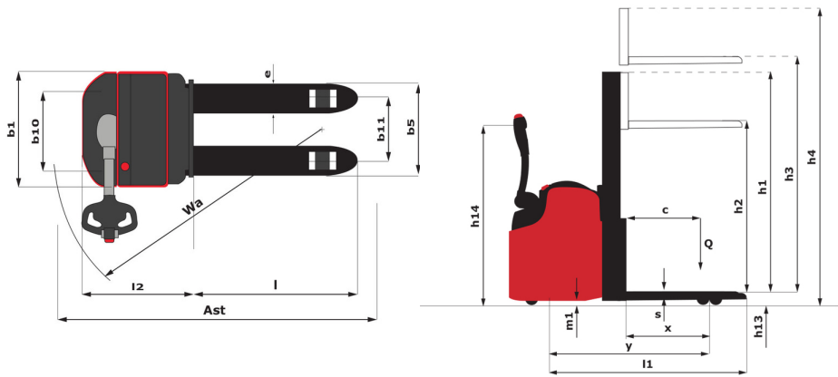
ES 614 - Dimensional drawing
