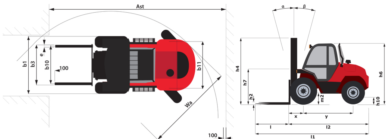
M-X 30-2 - Dimensional drawing
