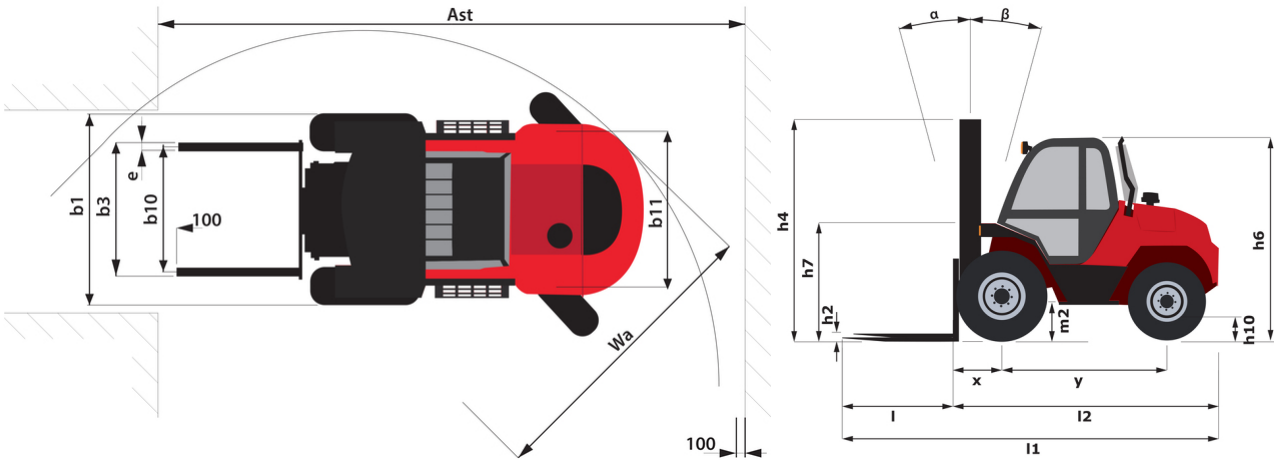
M-X 30-2 - Diagrama dimensional
