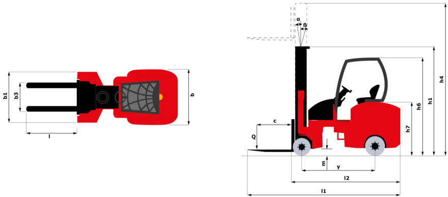
EMA II 18 HL-1 - Dimensional drawing
