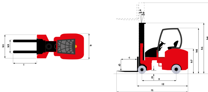
EMA II 20 HD-2 - Dimensional drawing
