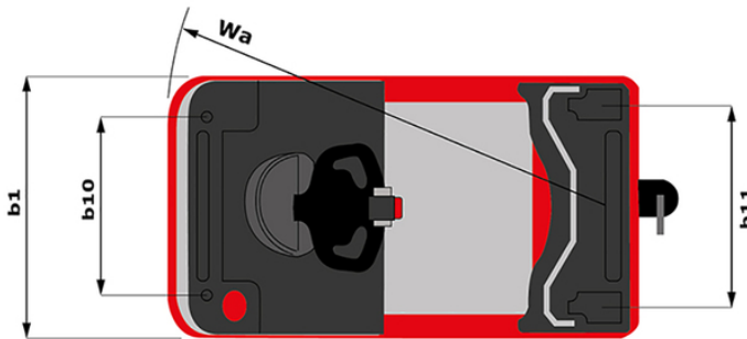
CT 50 - Dimensional drawing
