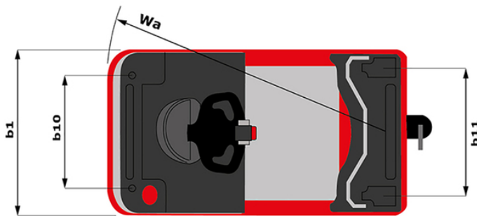
CT 50 - Diagrama dimensional
