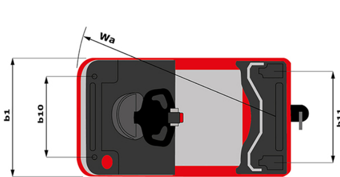
CT 50 - Diagrama dimensional
