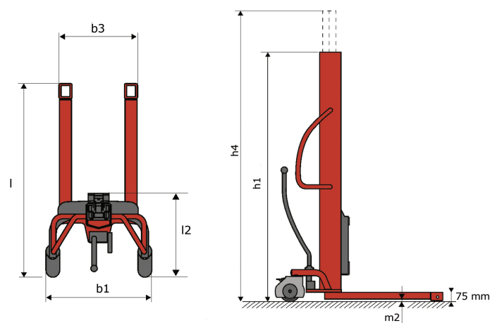
Kleos HM 500 D25 - Dimensional drawing
