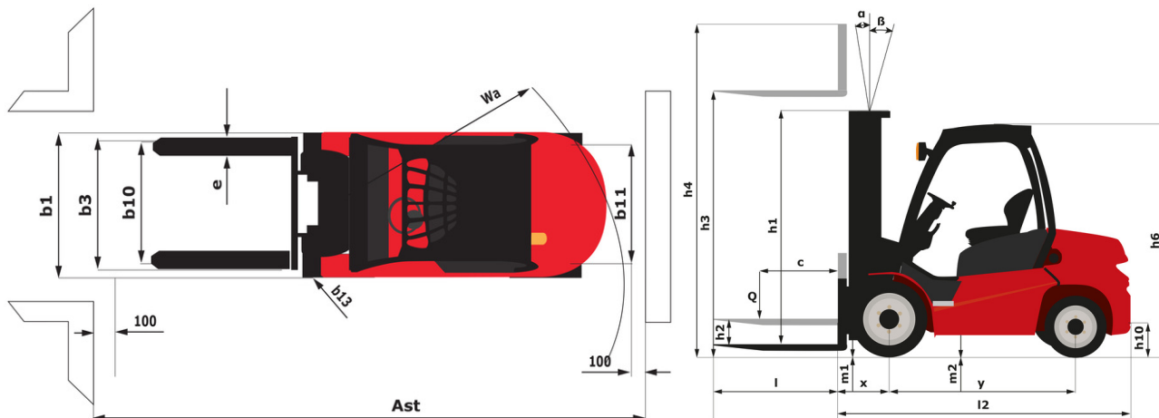
MI-X 50 L D - Diagrama dimensional
