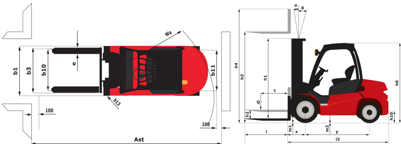
MI-X 60 D - Dimensional drawing
